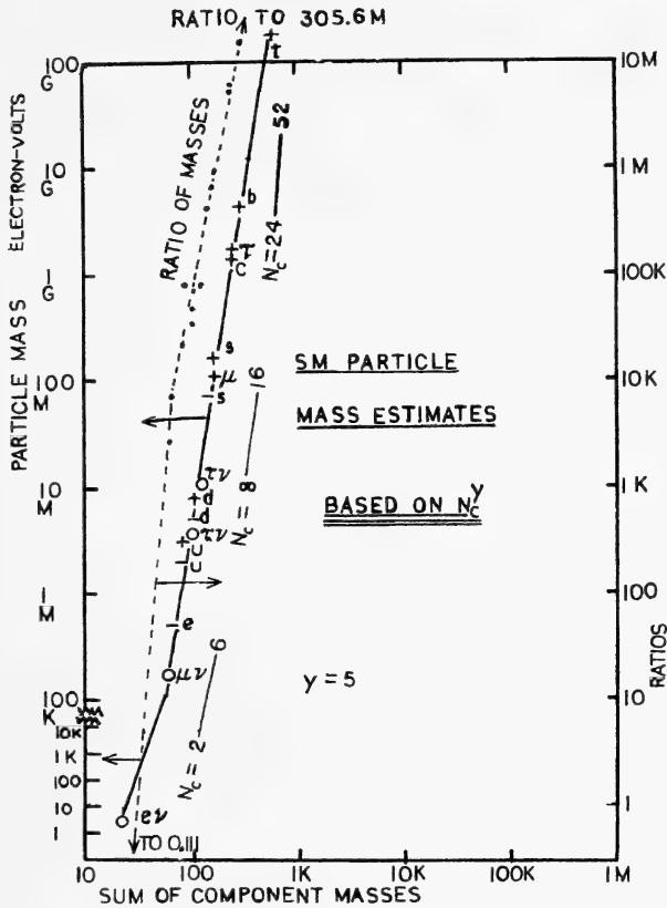
FIG. 2B. Separate view of the lepton and quark mass estimates graph in Fig. 2A. The ranges of numbers of quantal components required by the systematic regularity of these estimates is added.
